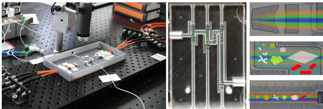
Figure 1 Photographs of a microfluidic lab-on-a-chip for the characterization of nano- and micro-suspensions by UV-NIR light extinction spectrometry
